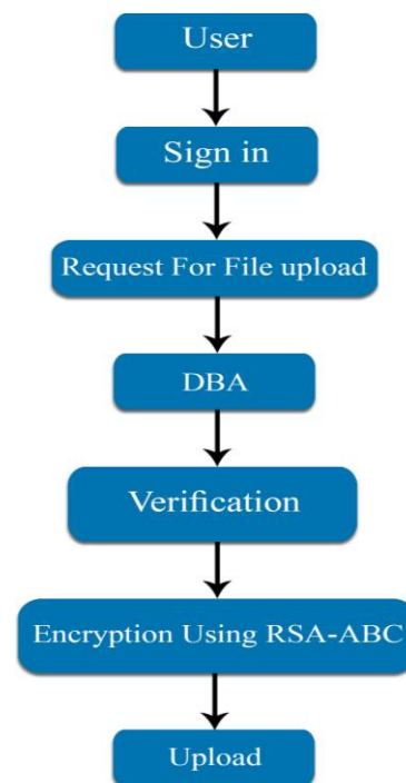
Figure.1 Proposed diagram for Hybrid RSA-MABC
